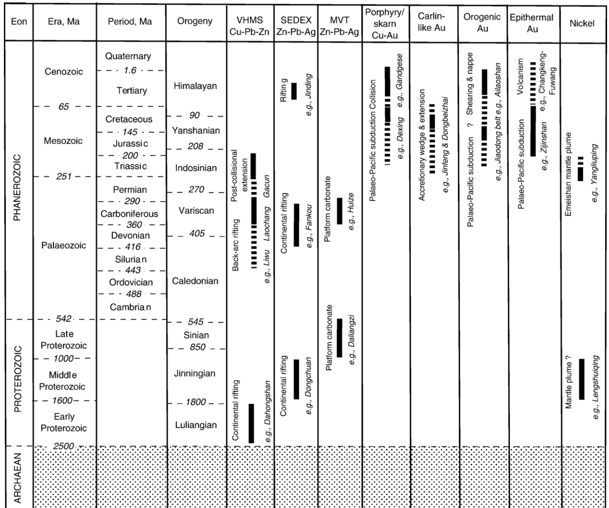
Fig. 15. Schematic diagram showing a simplified temporal evolution of the different deposit types in relation to tectonic and metallogenic events in South China. Multiple orogenic stages during the evolution of the South China Region were modified from Wang and Mo (1995) and Zhou Taihe et al. (2002).
