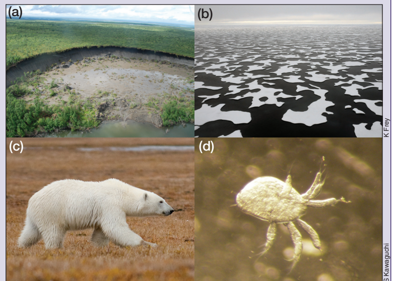
Figure 2. Examples of impacts of climate change in polar regions. (a) In terrestrial environments, thawing of ice-rich continuous permafrost, as shown here near the Mackenzie Delta in northern Canada, causes retrogressive thaw slumps. These land disturbances result in changes to surface water chemistry in adjacent rivers and lakes, alter local vegetation, and can damage infrastructure, such as pipelines for oil and gas, increasing the risk of point-source pollution. (b) Melting sea ice is reducing habitat for ice-dependent animals including (c) polar bears ( Ursus maritimus ) in the Arctic and (d) larval krill ( Euphausia superba ) in the Antarctic.
