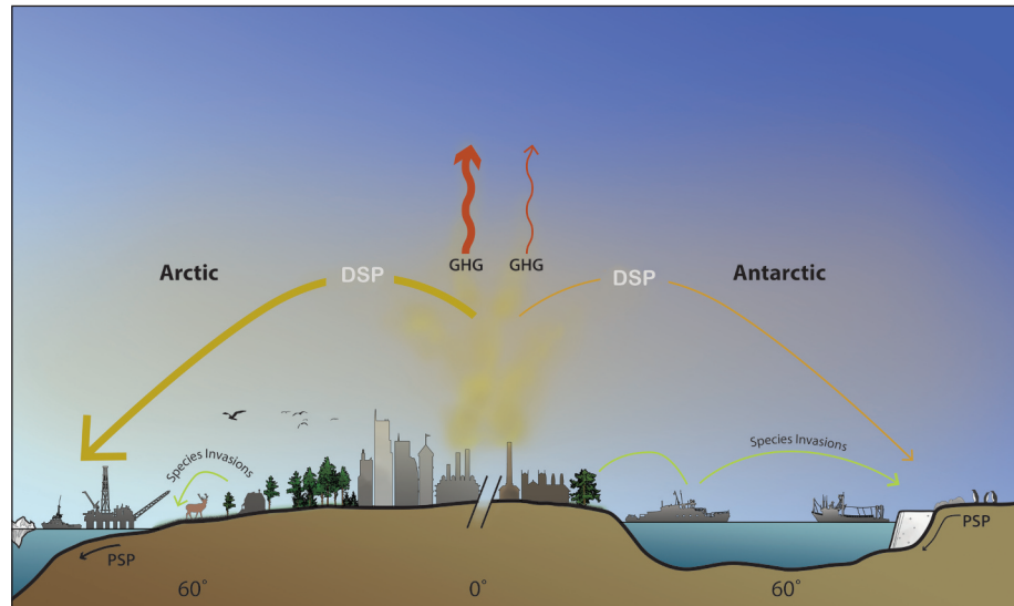
Figure 1. Shared threats to polar environments. Greenhouse gases (GHGs, red arrows) are the major causes of climate change, the principal threat to polar environments. Climate change interacts with other threats, including diffuse-source pollutants (DSPs) such as persistent organic pollutants and ozone-depleting chemicals that migrate from lower latitudes. It also raises the risk of more localized point-source pollutants (PSPs), as well as fisheries overexploitation (represented by fishing boats) and species invasions (green arrows).
