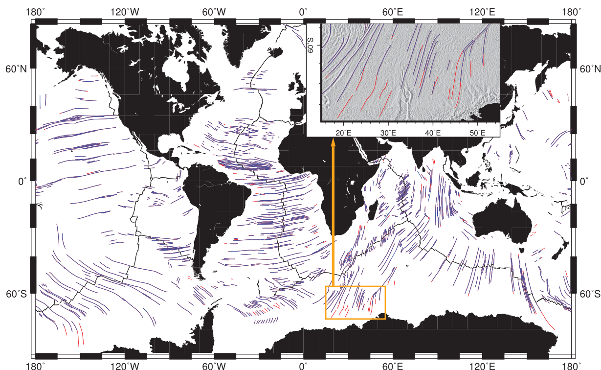
Figure 5. Red FZ strands show our recent improvements to the FZ compilation (blue) imitated by Matthews et al. [2011]. The reduced noise level in the VGG grid [Sandwell et al. , 2014] let us extend many FZs to older ages. See the GSFML web site for map of all seafloor fabric lineations.
