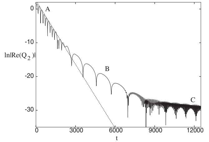
FIG. 2. Plot of \ln|\text{Re}(Q_2)| for a Gaussian vortex as a function of t . The dashed line gives the regime A decay rate \gamma_G = -0.0063 from a Landau pole calculation.
