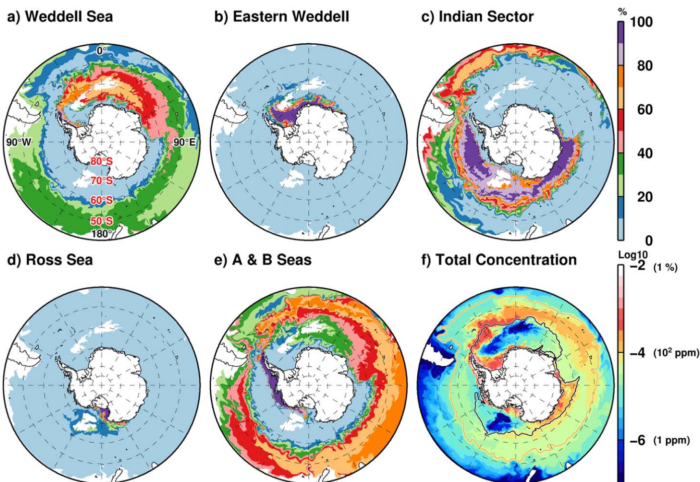
Figure 5. Horizontal distribution of basal meltwater tracers at the surface at the end of integration. (a–e) The percentage of the meltwater tracer of each ice shelf region to the total meltwater concentration in the Figure 5f. The area of the total tracer concentration smaller than 10^{-6} is masked out in the Figures 5a–5e. In the Figure 5f, the zero line of the transport stream function (as representatives of m-Bdy, black line) and m-SAF (orange line) are superimposed.
