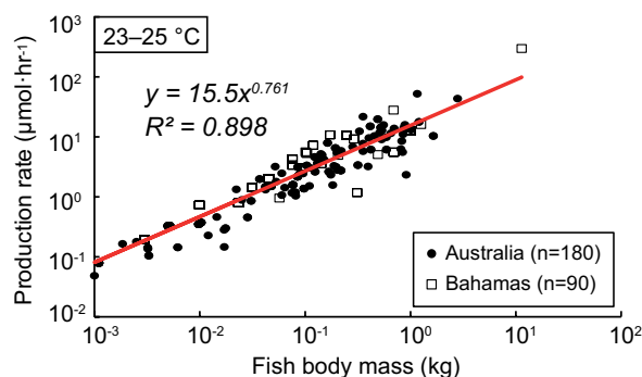
Figure 3. \text{CaCO}_3 production rate–body mass relationship at 23–25 °C, based on data from Australia (this study) and the Caribbean (Perry et al., 2011).
