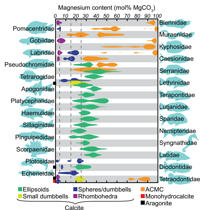
Figure 2. Magnesium content distributions (mol% \text{MgCO}_3 ) of Australian fish-derived low-Mg calcite (LMC), high-Mg calcite (HMC), and Mg-rich amorphous calcium carbonate (ACMC). Family-level results are a composite of data from each member (n = 1–4; see Table DR1 [see footnote 1]). Where products involve a variety of carbonate polymorphs/morphologies (e.g., family: Lethrinidae [emperors]), corresponding histograms are independent and do not show relative abundances.
