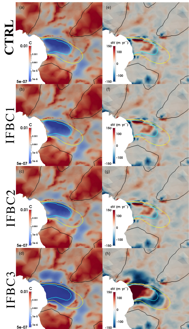
Figure 8. Distribution of basal friction coefficient C ( \text{MPa m}^{-1} \text{yr} ) (left column), and the mismatch between the observed and modelled surface velocity (observed minus simulated; right column) from experiments: (a, e) CTRL (first row), (b, f) IFBC1 (second row), (c, g) IFBC2 (third row), and (d, h) IFBC3 (fourth row). The black, yellow, and cyan solid lines represent surface speed contours of 100, 1000, and 1500 \text{ m yr}^{-1} , respectively.
