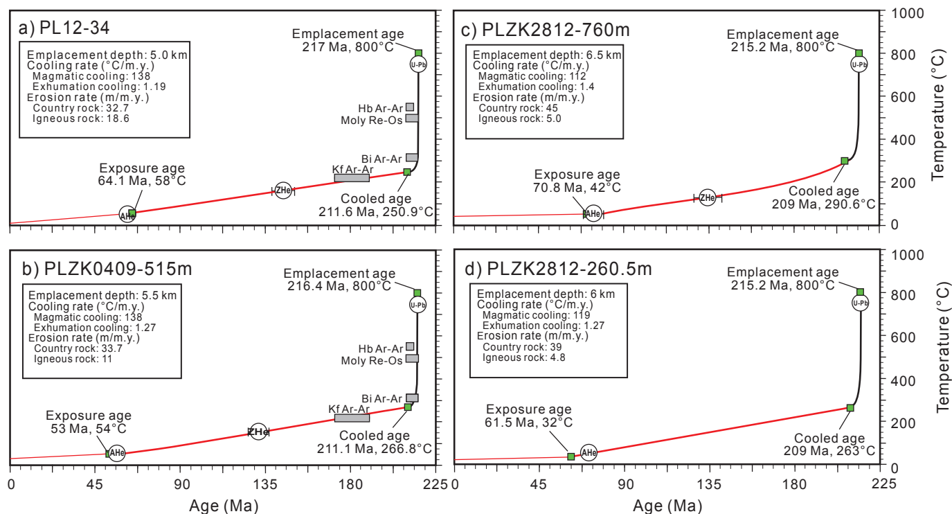
Fig. 6. (a-d) Graphic depiction of modeling results for some representative samples from the Pulang complex obtained using 4DTherm of Fu et al. (2010). The previously published Ar-Ar and Re-Os ages (Table 1) are also plotted in the left two figures for comparison. Abbreviations: AHe = apatite (U-Th)/He, Bi = biotite, Hb = hornblende, Kf = K-feldspar, Moly = molybdenite, ZHe = zircon (U-Th)/He.
