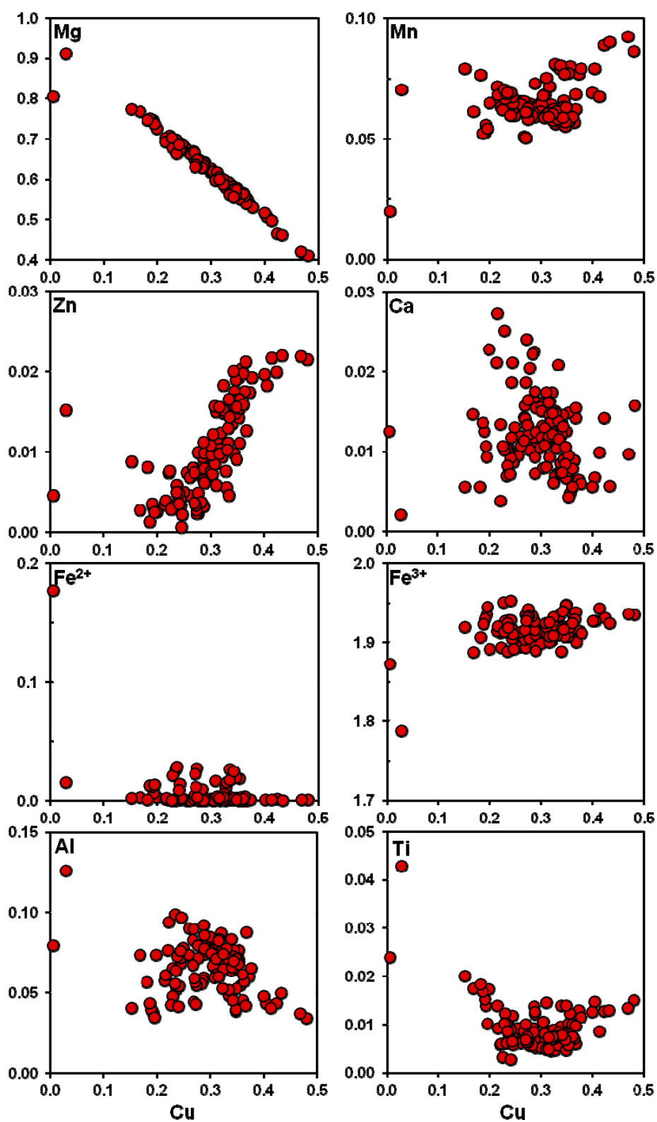
Figure 10. Variations of Cu vs. other elements (in apfu) for Cu-magnesioferrite from the Duplex lava tube, Tolbachik volcano, Kamchatka peninsula, Russia. Database of EMPA-WDS analyses (Table S6) were used.
