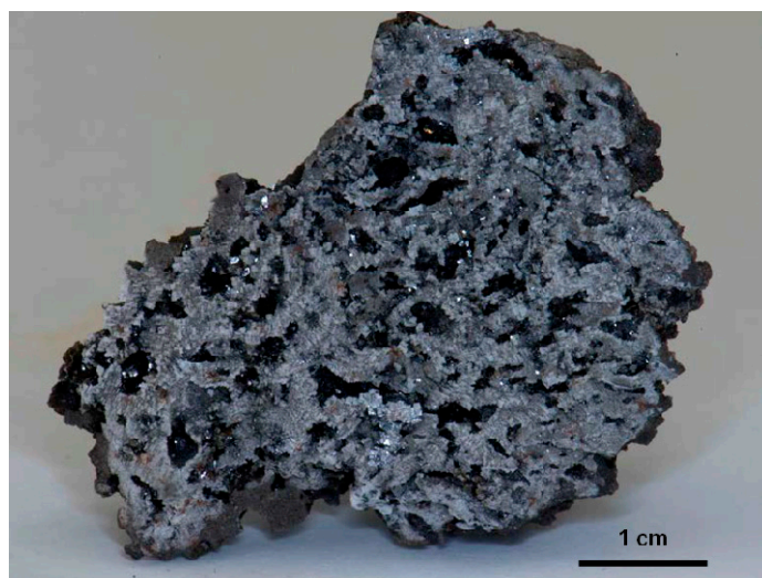
Figure 3. General view of sample from the lava wall covering by crystals of chlorides and tenorite, Duplex lava tube.
