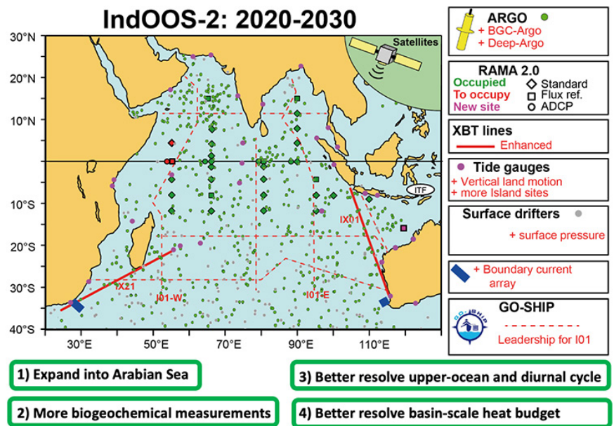
Fig. 8. Main IndOOS-2 recommendations. Argo: Maintain the core 3^\circ \times 3^\circ array; add 200 BGC-Argo floats; develop a Deep-Argo program. RAMA: New RAMA-2.0 design that better addresses operational constraints; occupy three remaining sites in Arabian Sea; increase resolution of upper-ocean measurements and add biogeochemical measurements at flux reference sites; add a new flux site off northwestern Australia. XBT: Maintain IX01 and IX21 lines, install autolaunchers, and increase near-coastal resolution on IX01. Tide gauges: Add collocated measurements of land motion; add sites in the southwestern Indian Ocean and on islands. Surface drifters: Maintain core 5^\circ \times 5^\circ array; evaluate addition of barometric pressure measurements. Boundary current arrays: Add measurements of mass, heat, and freshwater fluxes of the Agulhas and Leeuwin Currents, including hydrographic end-point moorings to capture basin-scale overturning. GO-SHIP: Find national commitment for IO1-E and IO1-W sections; add measurements of phytoplankton community structure. Satellites: Maintain overlapping, intercalibrated missions; enhance spatial resolution of SSH or currents directly. These recommendations can be summarized in four core findings of the review, listed in green in the frames beside the map.
