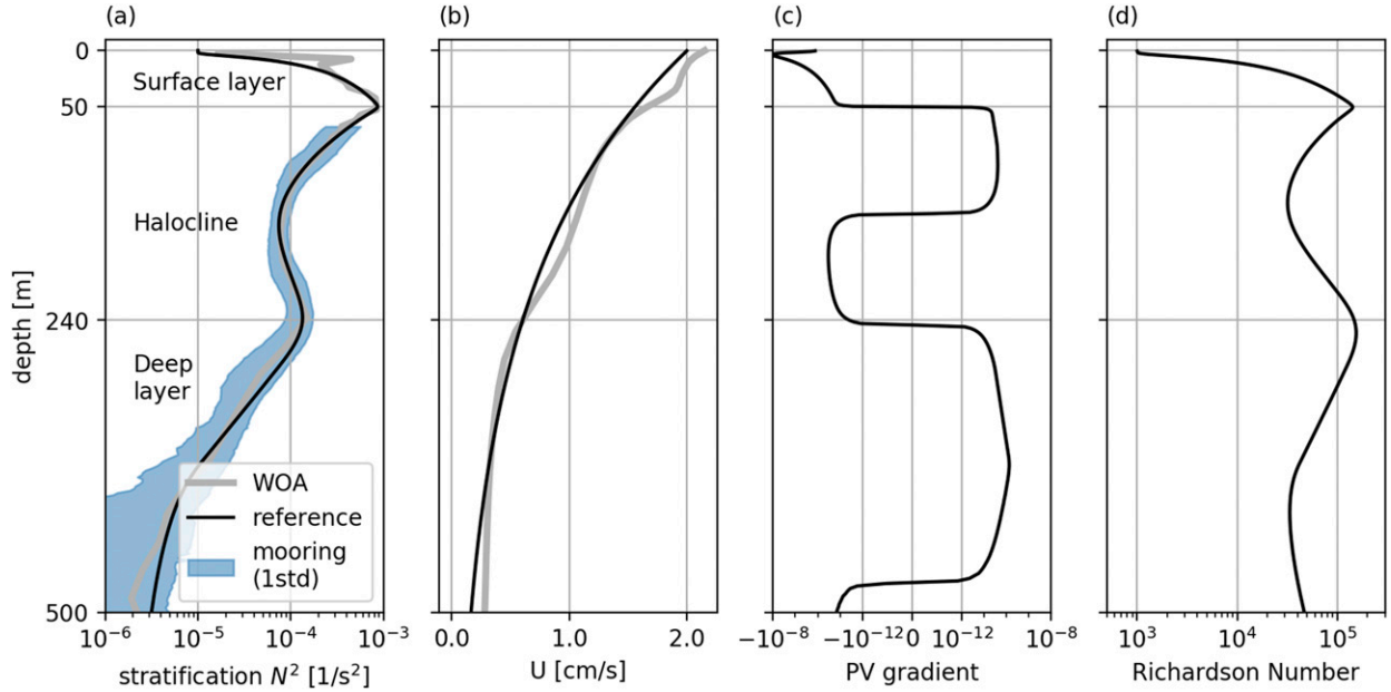
FIG. 3. Profiles of (a) stratification N^2 and (b) current speed U used for the baroclinic instability analysis (black curves) and the corresponding (c) quasigeostrophic PV gradient and (d) Richardson number Ri = N^2/(\partial U/\partial z)^2 . The blue shaded area in (a) is the same as Fig. 1. Gray thick lines show profiles computed from salinity and temperature fields from the 2005–17 World Ocean Atlas climatology at 75^\circ\text{N} , 150^\circ\text{W} . The corresponding quasigeostrophic PV gradient is too noisy and is not shown. Both stratification and velocity profiles used in our analysis extend from the surface to the ocean floor at a depth of 3800 m, but only the top 500 m are shown here.
