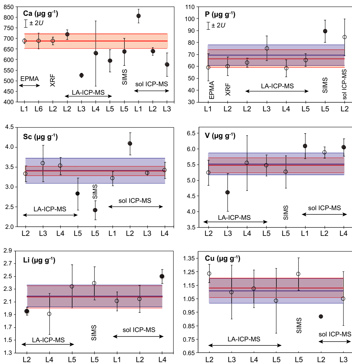
Figure 4. Mass fractions of Ca, P, Sc, V, Li and Cu obtained by different analytical techniques in different institutions. Symbols and horizontal lines as in Figure 3.
