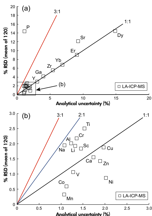
Figure 2. Assessment of homogeneity of olivine Mongol Sh11-2 on the basis of LA-ICP-MS analyses of 120 individual olivine fragments. Values of homogeneity index of 1 (black lines), 2 (blue line) and 3 (red lines) are shown. (a) The full range of values; note that P is the only element showing substantial heterogeneity. (b) Elements with % RSD values < 3%. See text for details.
