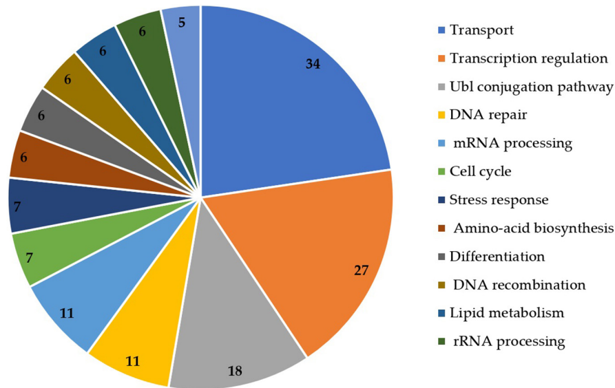
FIGURE 4 | Functional annotation of DEGs obtained from UniProt database.
