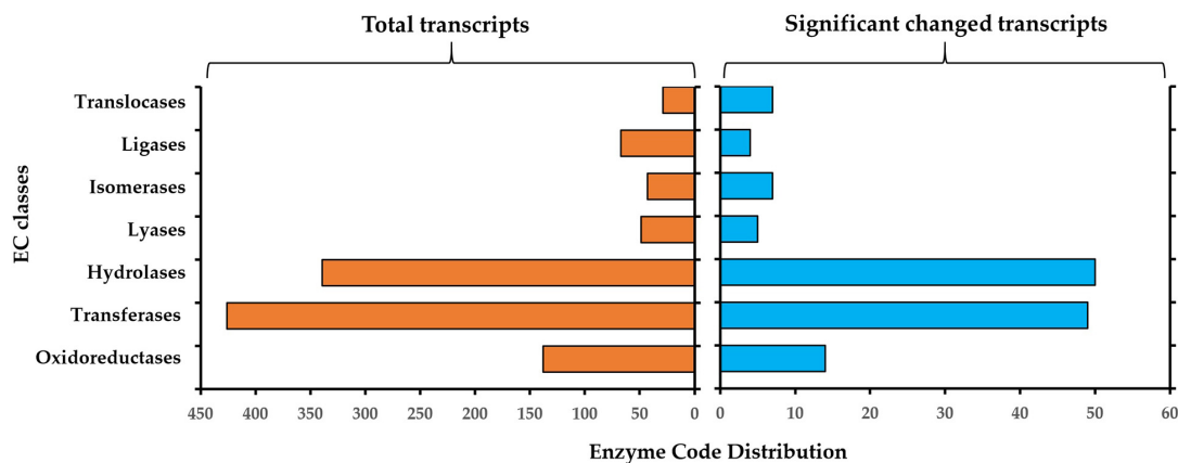
FIGURE 5 | Enzyme classification (EC) codes for the total (left) and significantly changed transcript (right) upon S. Subterranea spore germination. Note that one transcript can be associated with more than one EC term.
