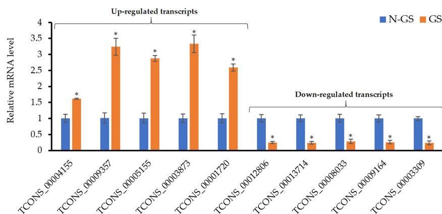
FIGURE 6 | Validation of RNA-Seq results using qRT-PCR. Values are the means of three biological replicates \pm SD. Asterisk (*) denotes a significant mRNA difference between germinating (GS) and non-germinating spore (N-GS) for each gene ( P -value < 0.01).
