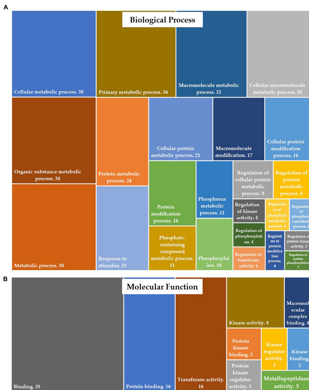
FIGURE 3 | Distribution of DEGs into gene ontology (GO) categories, according to (A) their involvement in biological processes and (B) their molecular function.
